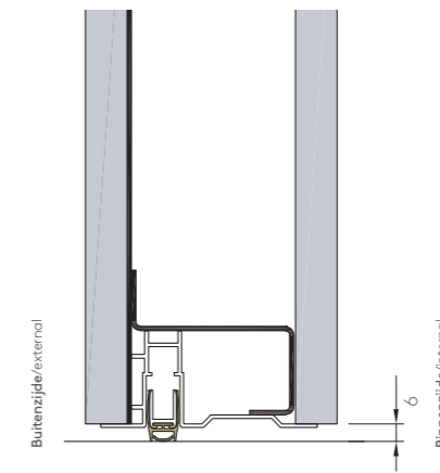
Standaard valdorpel | standard draught excluder
