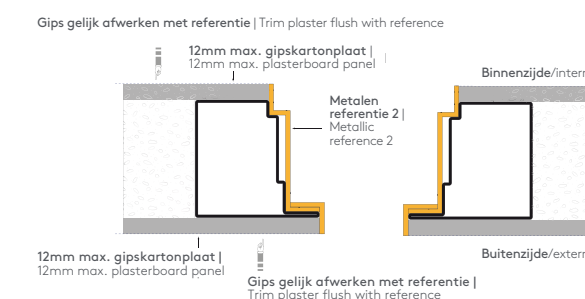
Vlak met binnen- of buitenwand Flush with internal/external wall
